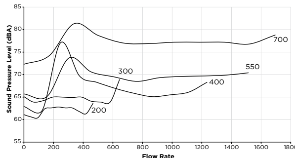
Sound Levels
