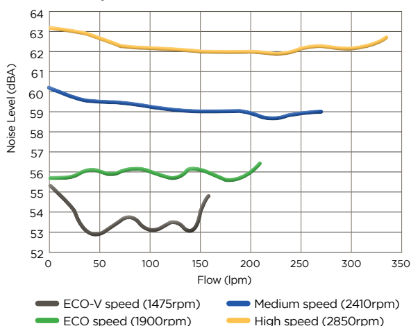
Hydrostorm ECO-V 100 Noise Levels
