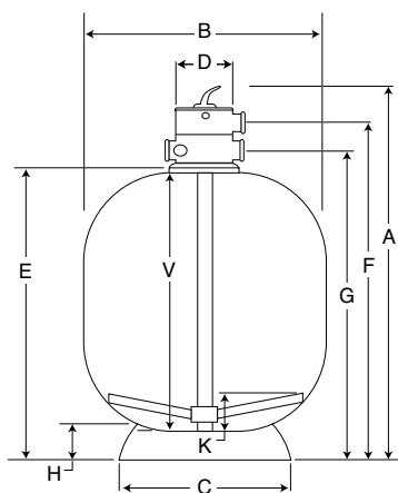
Lateral under drain system
