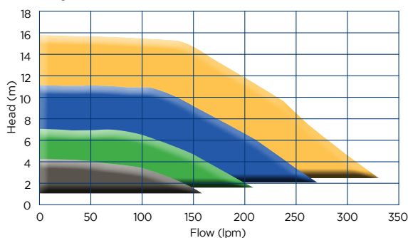
Hydrostorm ECO-V 100 Performance Curves
