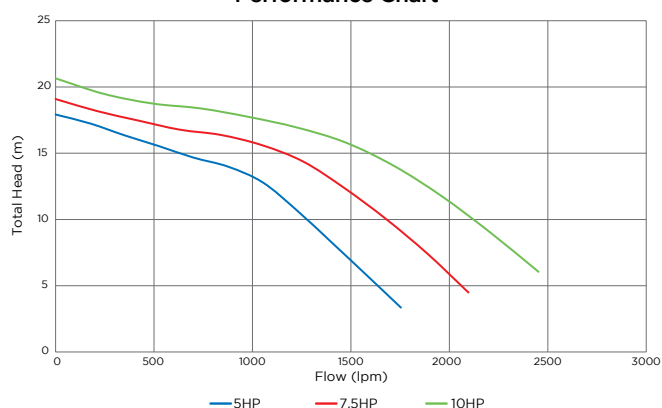
Performance Chart
