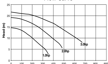
Flow Curve
