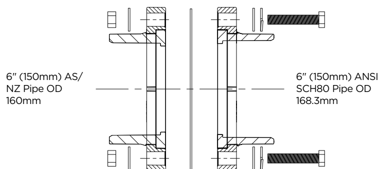
12161507 - 6" ANSI to 6" AS/NZ flange adapter kit
