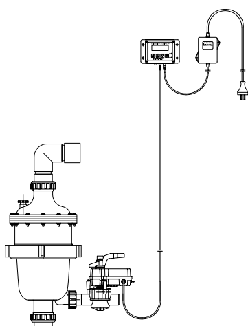
MultiCyclone 12/16 Auto Purge System 1 actuator
