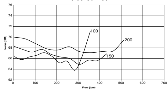
Noise Curves
