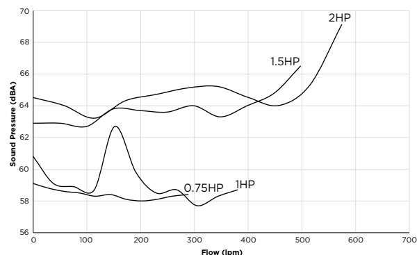
Alphaflo Sound Levels
