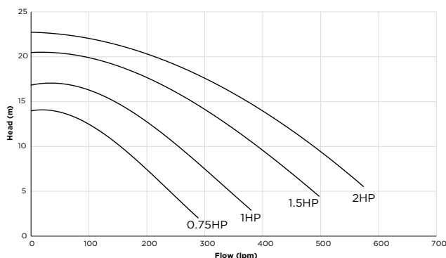
Alphaflo Flow Curves
