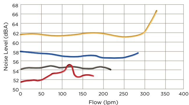
Supatuf MK2 ECO-V 100 Noise Levels
