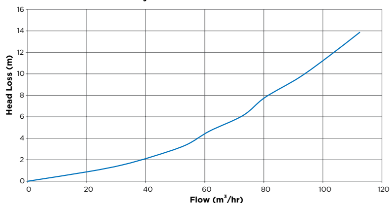
MultiCyclone 70XL Head Loss Curve
