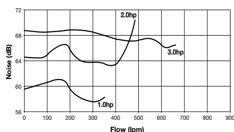
Sound Levels
