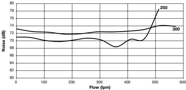
Hydrostorm Plus Sound Levels
