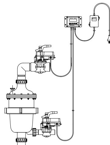
MultiCyclone 12/16 Auto Purge System 2 actuators
