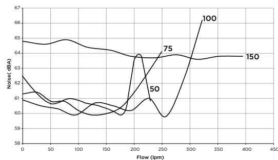
Noise Levels
