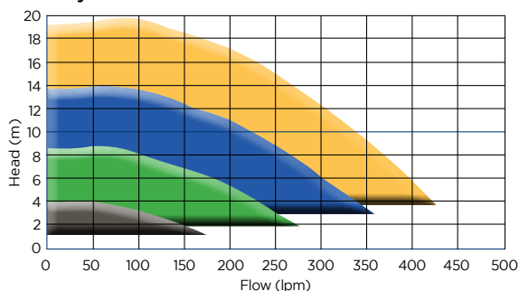
Hydrostorm ECO-V 150 Performance Curves
