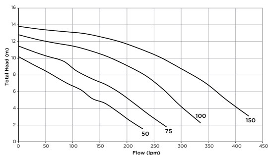
Flow Curves
